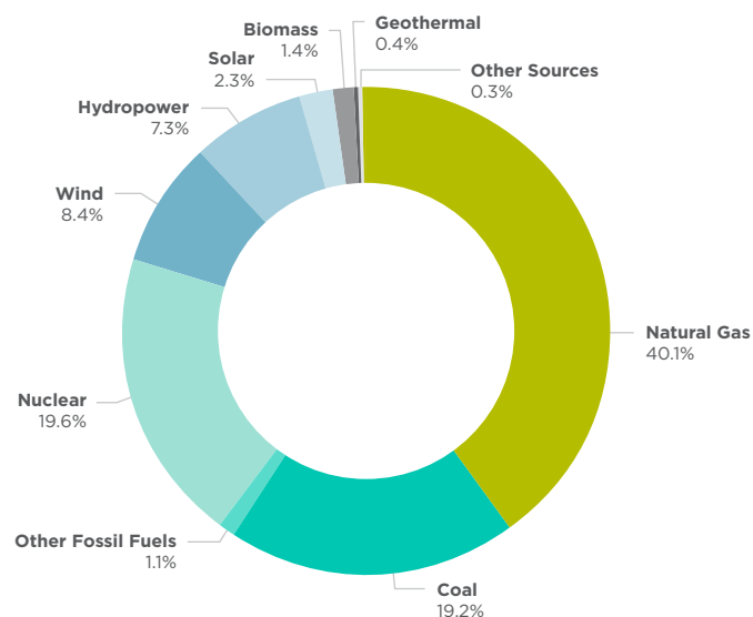
FIGURE 1. U.S. Utility-scale Electricity Generation by Source, 2020 6
