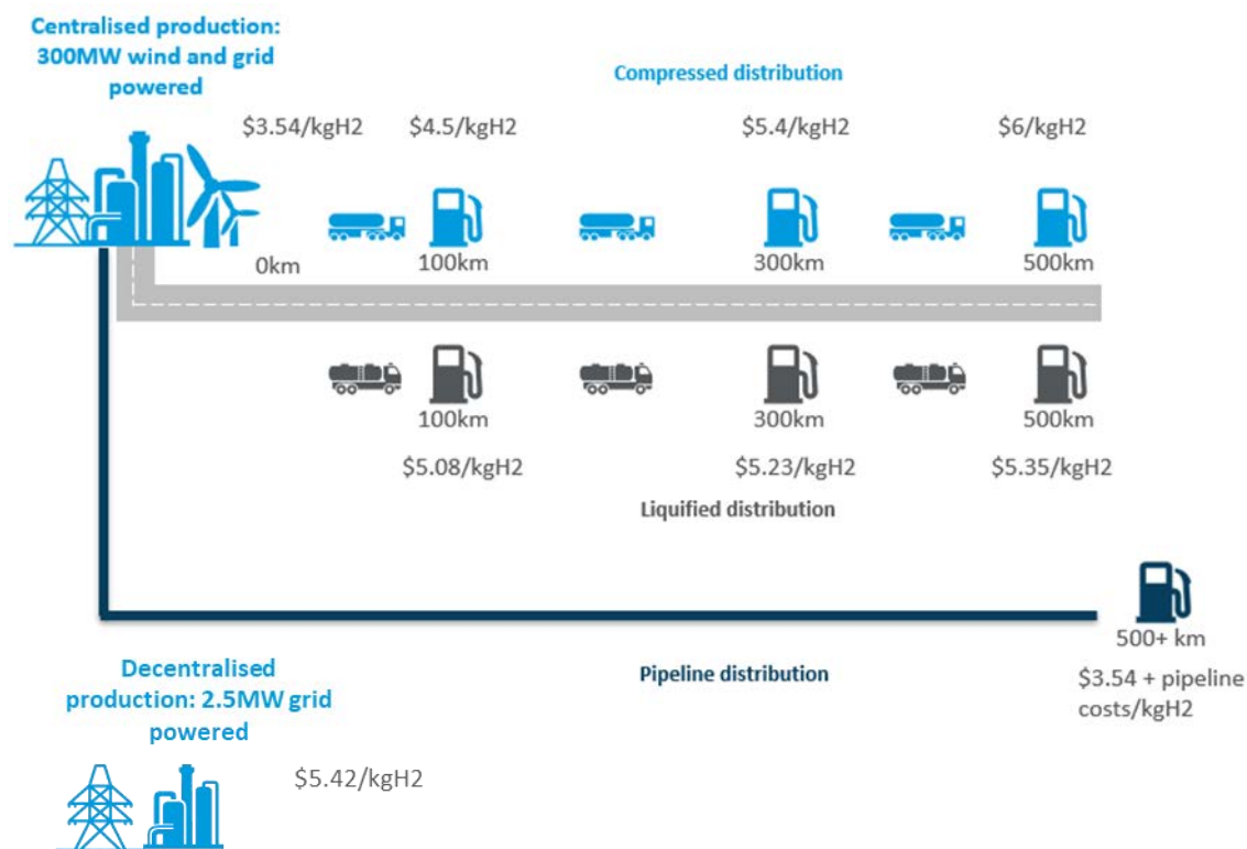
Figure 0.1: Illustration of centralised vs decentralised production in 2035 under BAU (US$)
