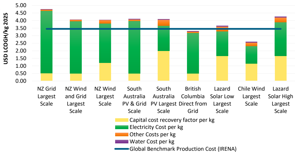
Figure 4.10: Comparison of New Zealand and overseas production costs in 2025
