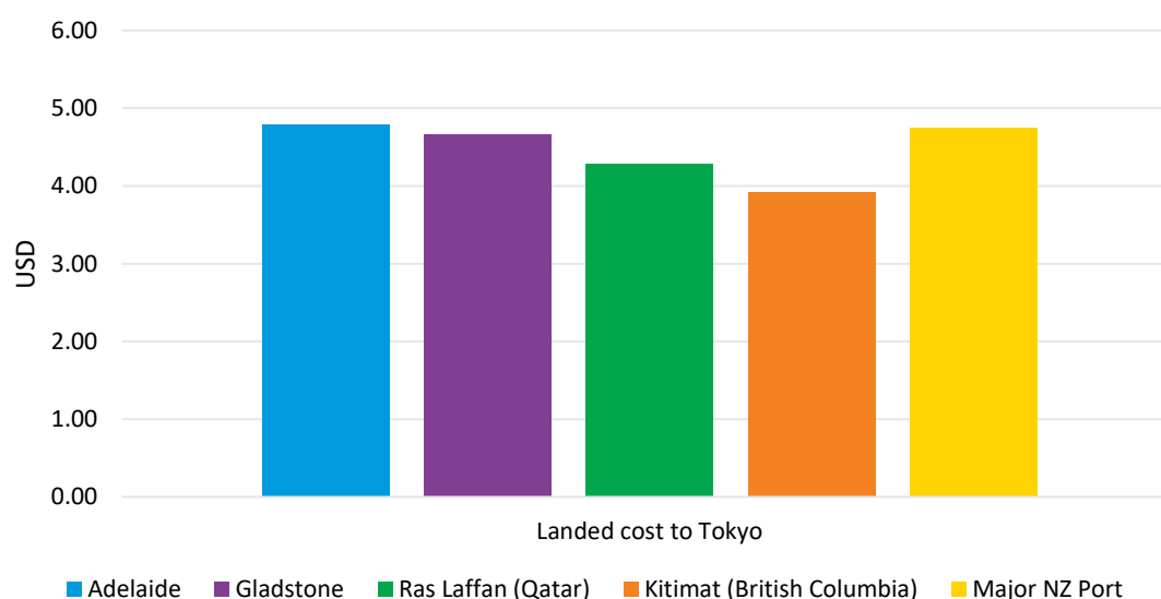
Figure 4.11: Comparison of landed hydrogen costs to Tokyo, Japan (2035)
