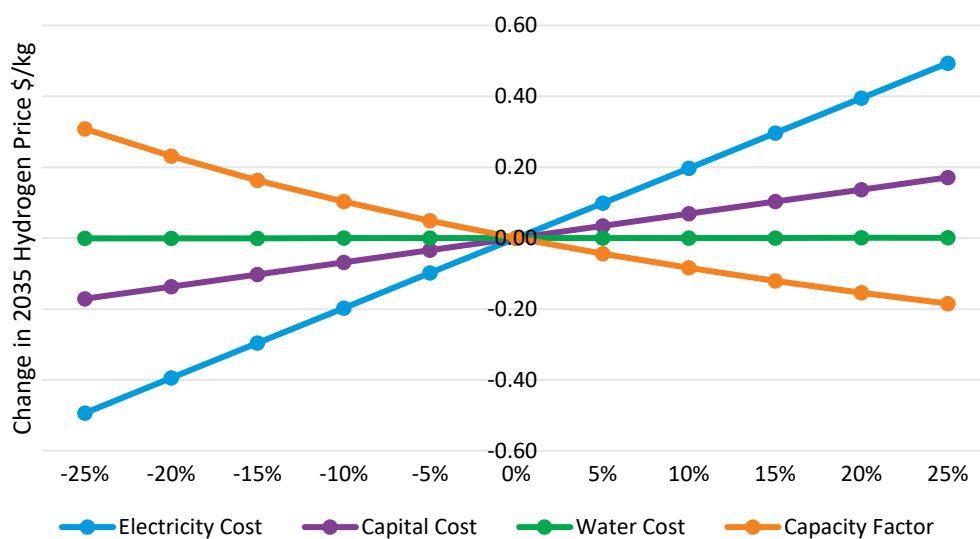
Figure 4.3: Sensitivity of hydrogen production at scale to inputs
