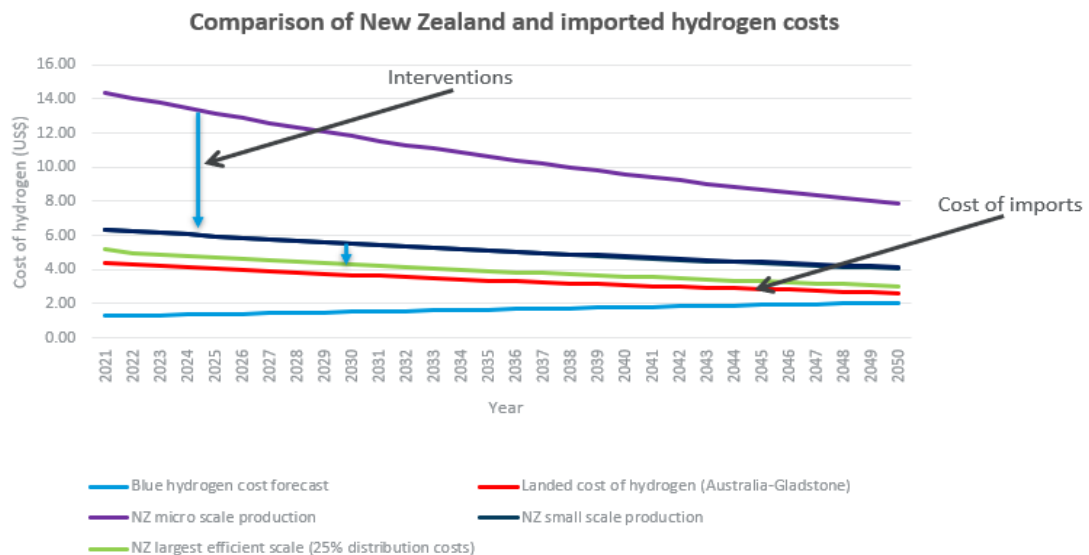
Figure 5.7: Comparison of New Zealand and imported green hydrogen costs
