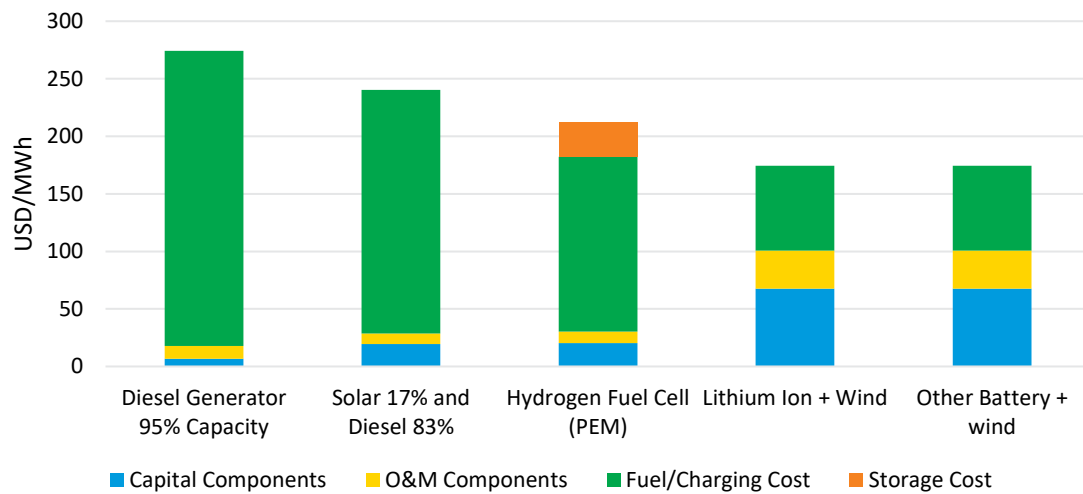
Figure 4.8: Comparative energy costs of different electricity production and storage technologies in 2050 for 1MW isolated systems
