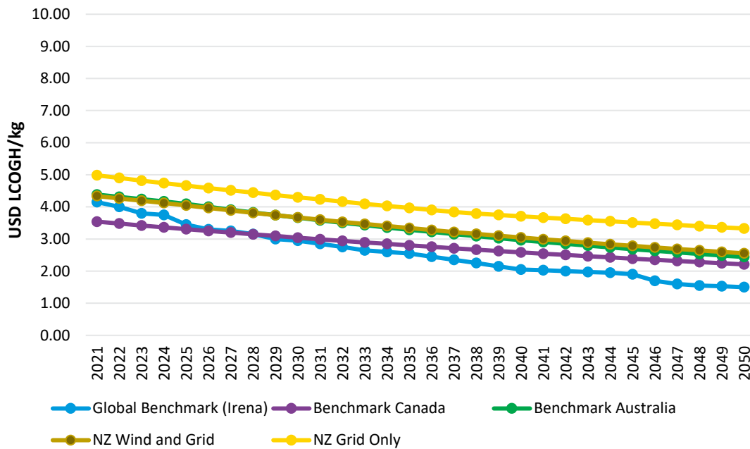
Figure 4.4: New Zealand and global comparator hydrogen production costs
