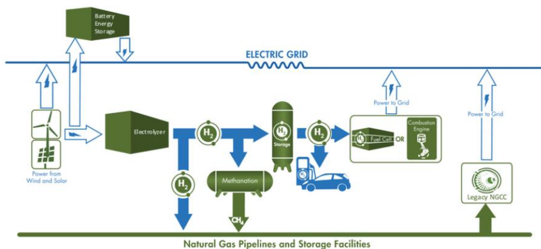
Figure 3.2: P2G and hydrogen energy storage
