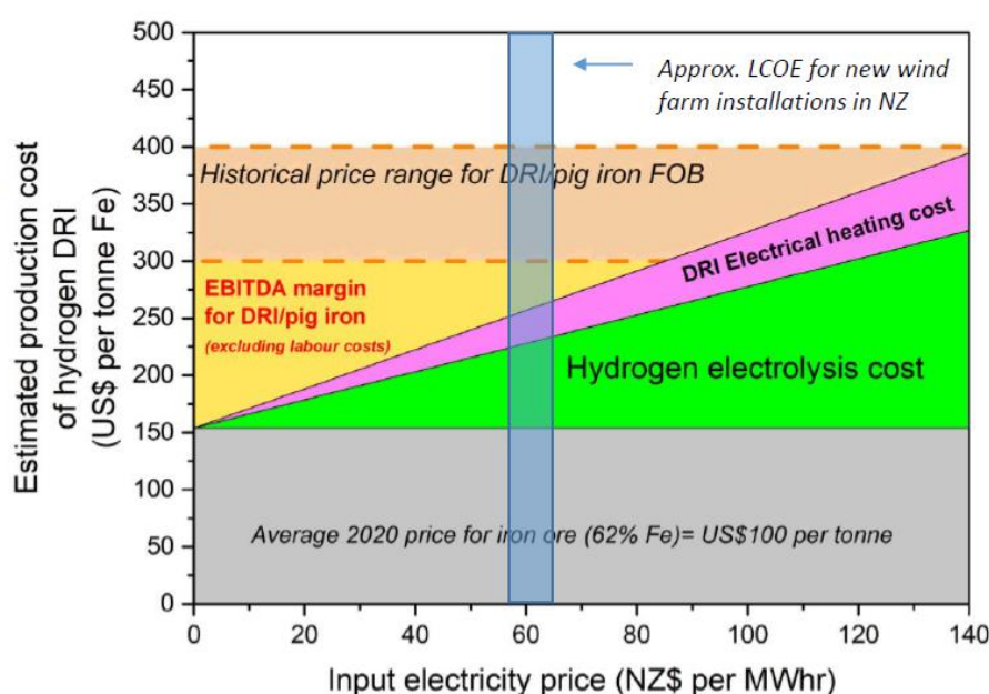
Figure 4.9: Illustration of DRI steel production costs and implied electricity cost
