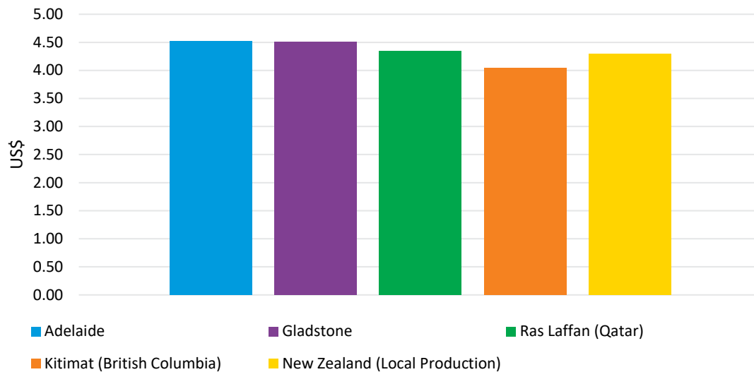
Figure 5.6: Landed costs of hydrogen to Auckland or Lyttleton compared to local production (2035)
