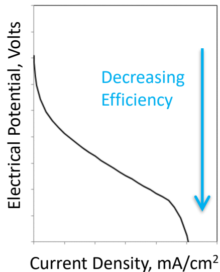
Fuel Cell Performance
