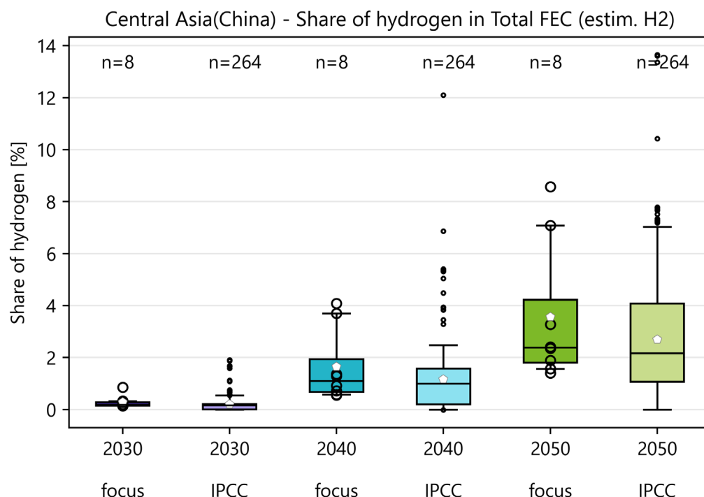
Figure 43: Central Asia - Total demand - Share of hydrogen
