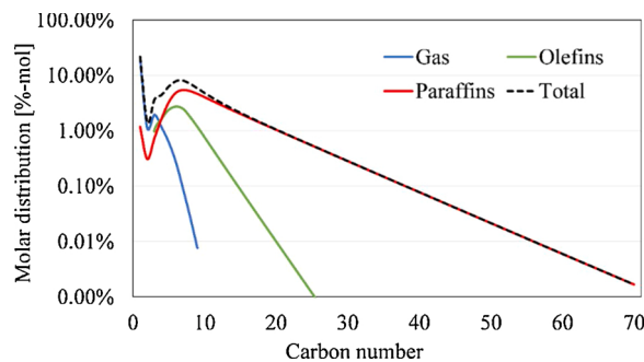
Fig. 3. FT products distribution of C.1: global FT distribution (black dashed line) and break-down of the products' components.
