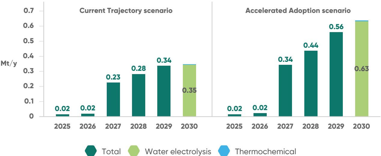
FIGURE 3.14 Electrolytic supply scenarios by 2030 and NECP or strategy targets
