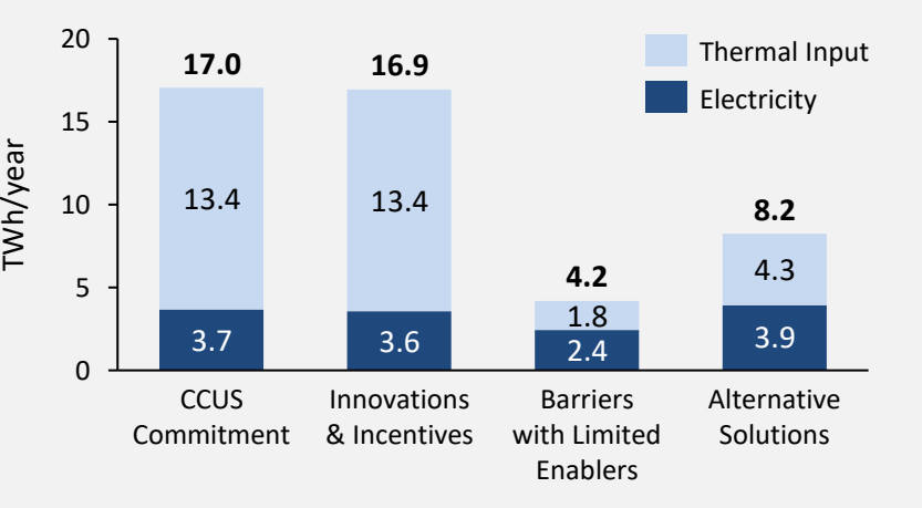
Chart 5.12 Energy requirements for Carbon Capture in 2040
