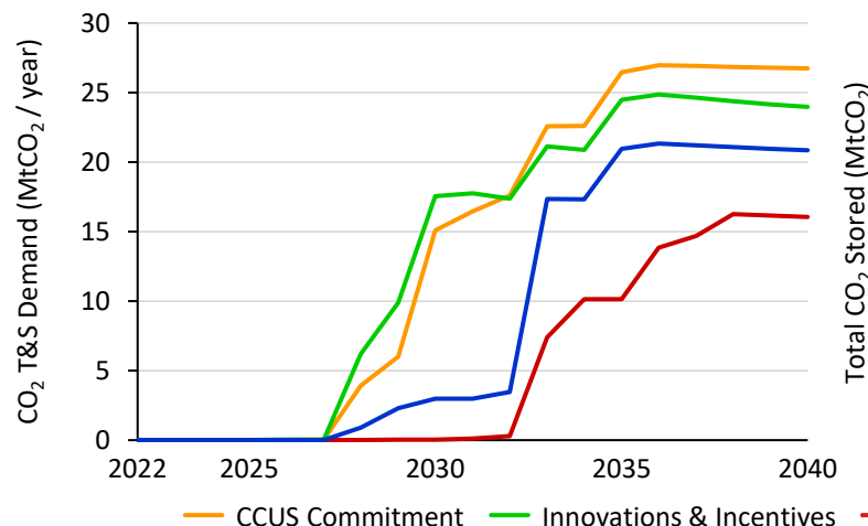
Chart 5.1 CO 2 annual T&S demand for carbon capture (cluster + blue H 2 )
