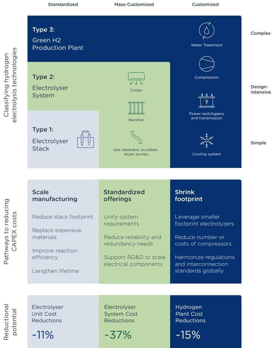
Figure 19: Achieving lower capital expenditure costs for each type of technology used in hydrogen production plants.
