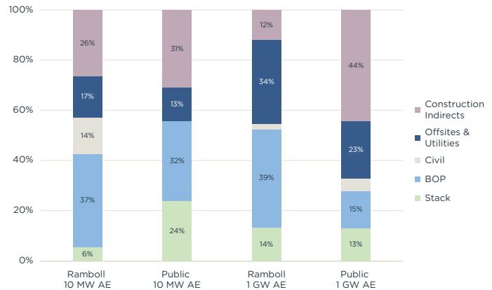
Figure 12: Ramboll vs. Public Estimates of AE System Components at scale (non-pressurized system).
