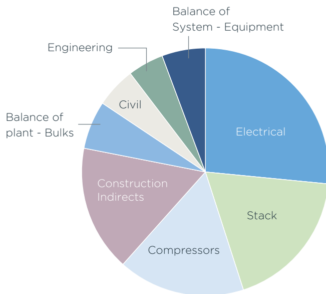
Figure 17: Ramboll's estimates show that local requirements for interconnections to power and offtake systems, such as electrical (grid connection, resiliency, power quality), compressors, and other balance of plant components drive a higher share of CAPEX than public estimates, even at larger (100+ MW) scales.
