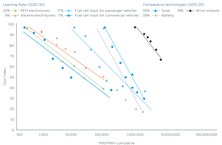
Figure 5: Hydrogen Council's Estimation of Learning Rates for Hydrogen and Clean Energy Production Technologies 14
