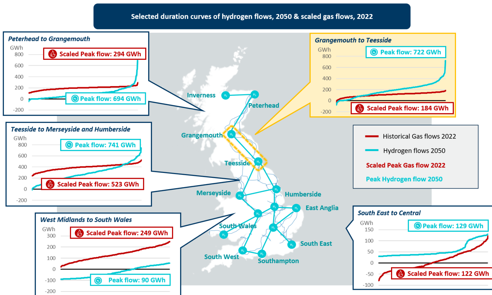
Figure 8-4: Selected daily duration curves of hydrogen flows (GWh), 2050 &amp; scaled daily 2022 gas flows (GWh), 2022
