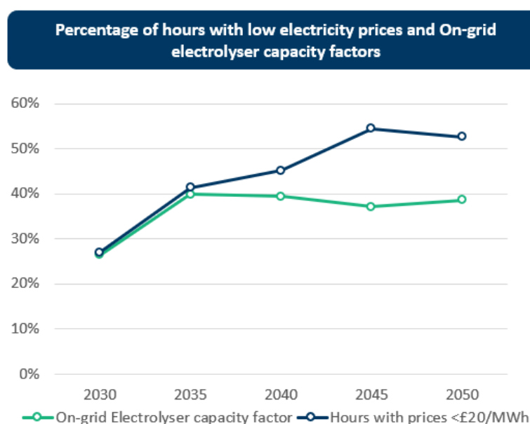
Figure 7-1: Percentage of hours with low electricity prices and On-grid electrolyser capacity factors
