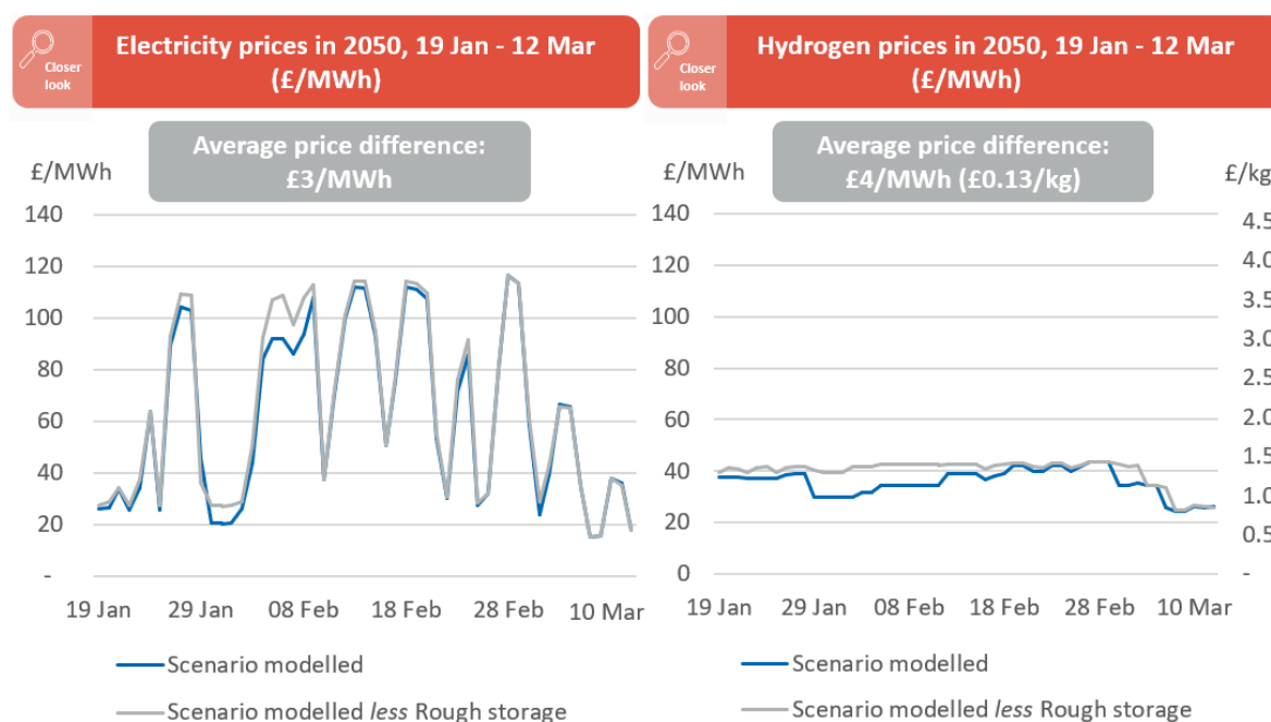
Figure 8-9: Wholesale hydrogen and wholesale electricity prices in 2050, 19 Jan to 12 Mar
