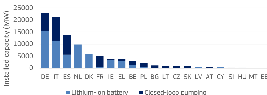
Figure 18: Closed-loop pumping and lithium-ion batteries installed capacity in the MIX-H2 scenario for the year 2030
