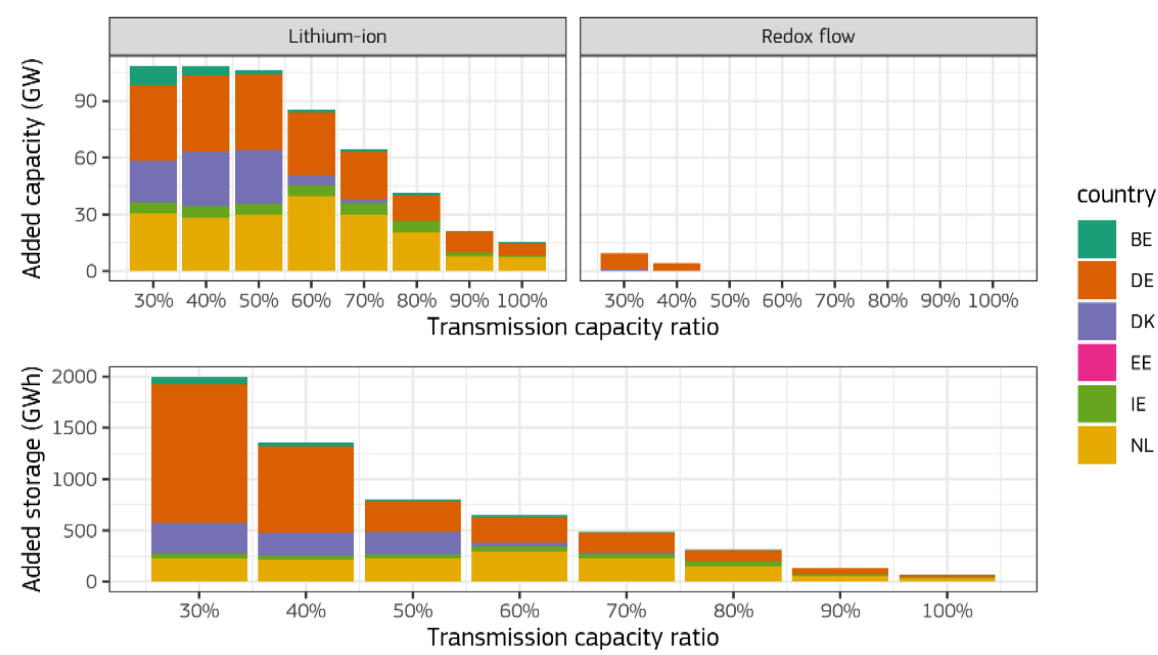
Figure 21: Top panel: Additional battery capacity per country and technology with respect to the variation of the capacity of electricity interconnectors. Bottom panel: total added storage (including all the selected technologies) per country. All the results are based on the MIX-H2 2030 scenario.
