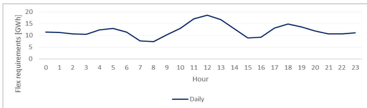
Figure 7: Average hourly summed (positive and negative) flexibility requirements in the EU in 2030.
