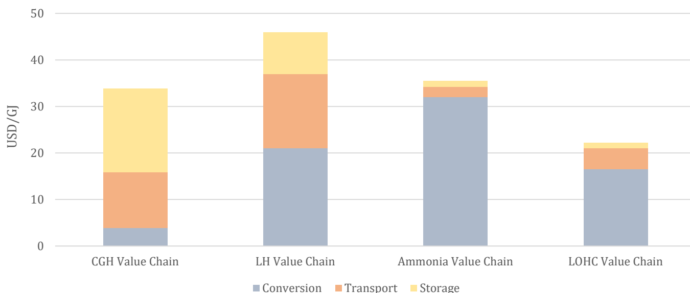
Figure 8 Global cost of energy penalty from four hydrogen value chains
