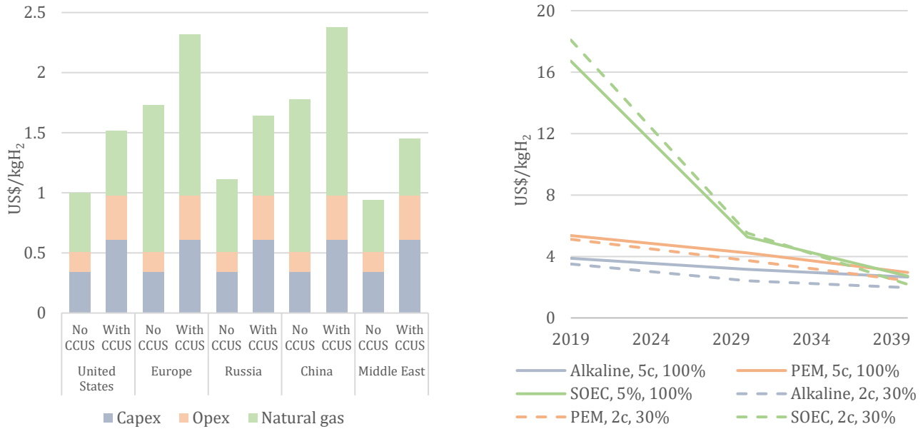
Figure 6 Hydrogen production costs using natural gas 26 versus hydrogen production costs using electrolysis 27
