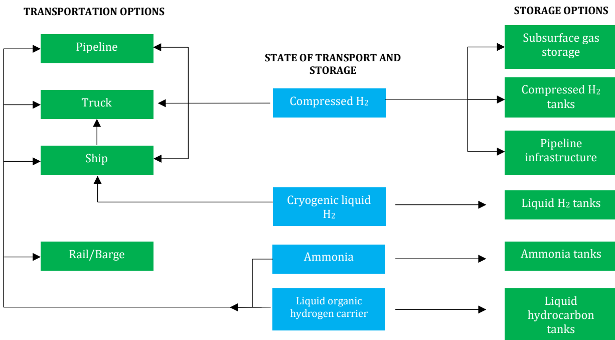
Figure 7 Main options for H 2 storage and transport 28
