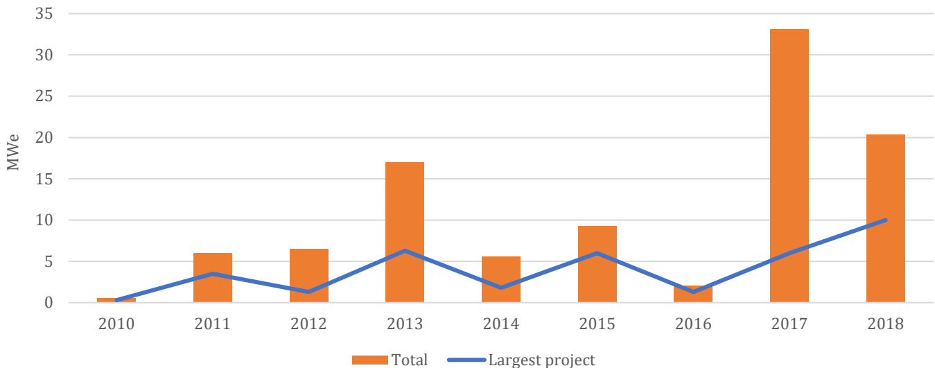
Figure 4 Global annual installation of electrolyser capacity, 2010-18
