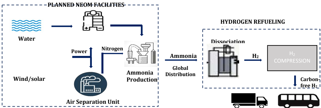
Figure 15 Neom planned H 2 production, transport and application
