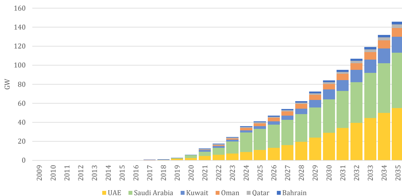
Figure 12 Installed and planned solar (Photovoltaic + Concentrated Solar) Power capacity in the GCC
