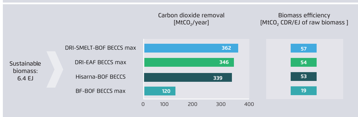
Carbon dioxide removal potential of various BECCS technologies in the steel sector for 6.4 EJ of sustainable primary biomass use
