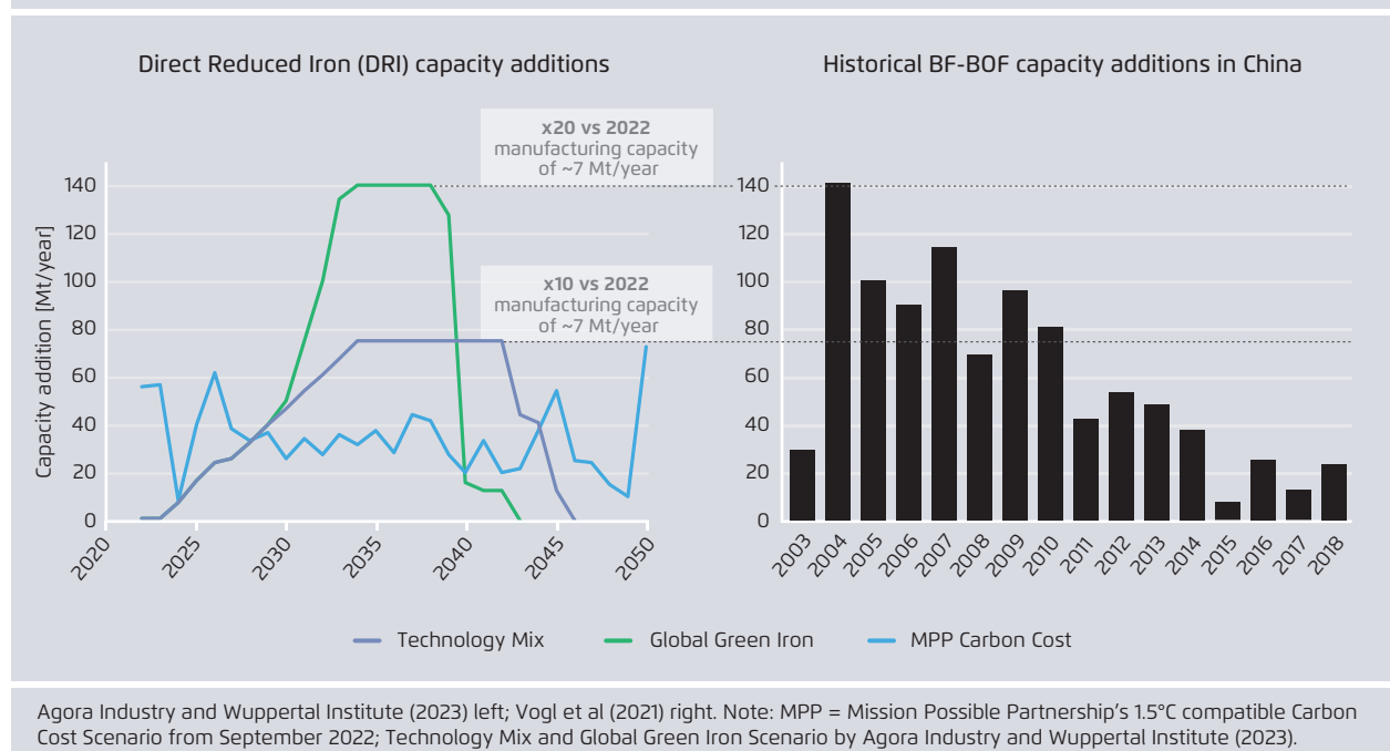
A massive scale-up of DRI is necessary to accelerate the global steel transformation
