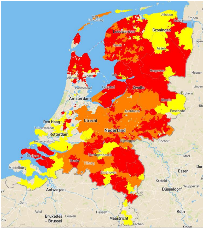
Figure 46 Capacity map of the Dutch electricity grid as of 14/04/2022 (injection) 221
