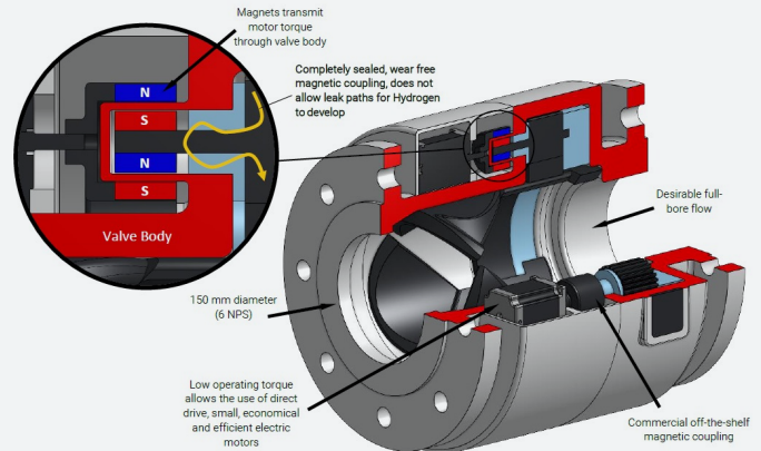
Figure 12: Dragonfly Valve
