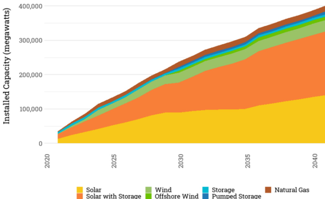
Figure 15: Projected Renewable Electricity Generation Additions Across Western States to Meet Clean Energy Targets 63
