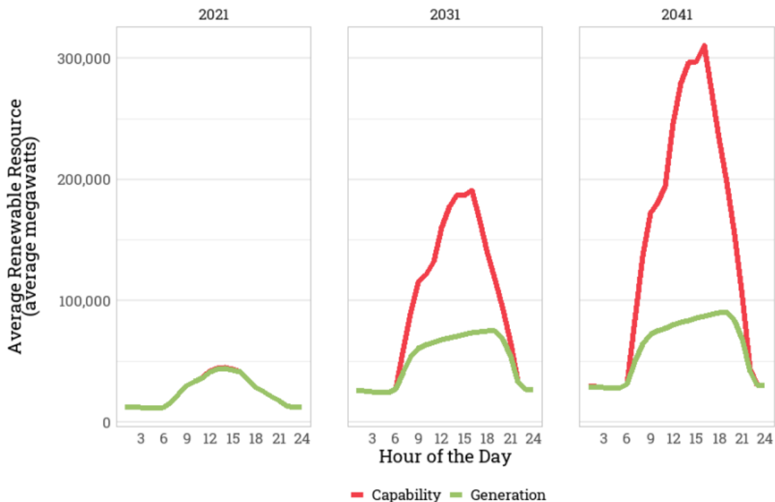
Figure 29: Future Renewable Resources and Curtailment in the Western Electric Grid 63
