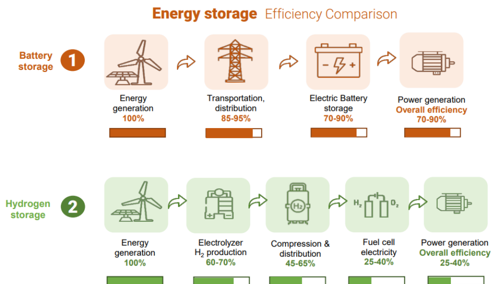
Figure 19: Efficiency Comparison of Energy Storage Using Batteries Versus Hydrogen 50
