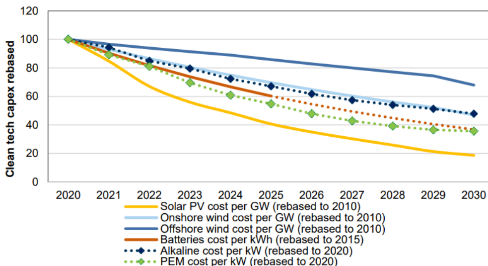
Figure 30: Forecasted Cost per kW for Electrolyzers and Renewables and kWh for Batteries 50
