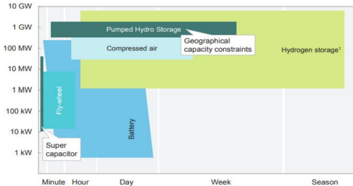
Figure 20: Capacity Versus Discharge for Energy Storage Technologies 50
