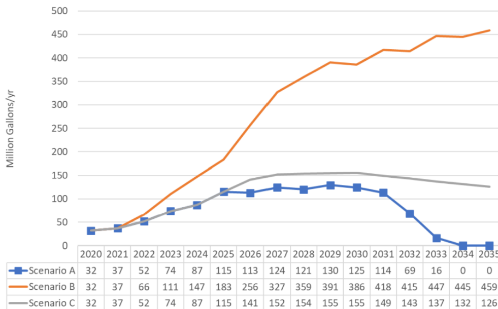
Figure 18: Renewable Diesel Volumes in the Oregon Clean Fuels Plan by Modeling Scenario 95
