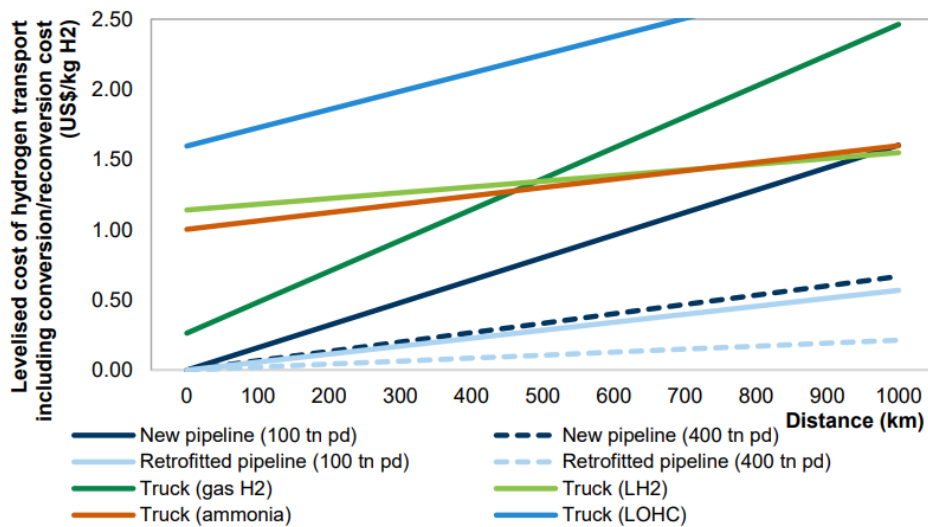
Figure 7: Levelized Cost of Hydrogen Transport Including Conversion/Reconversion Costs 50
