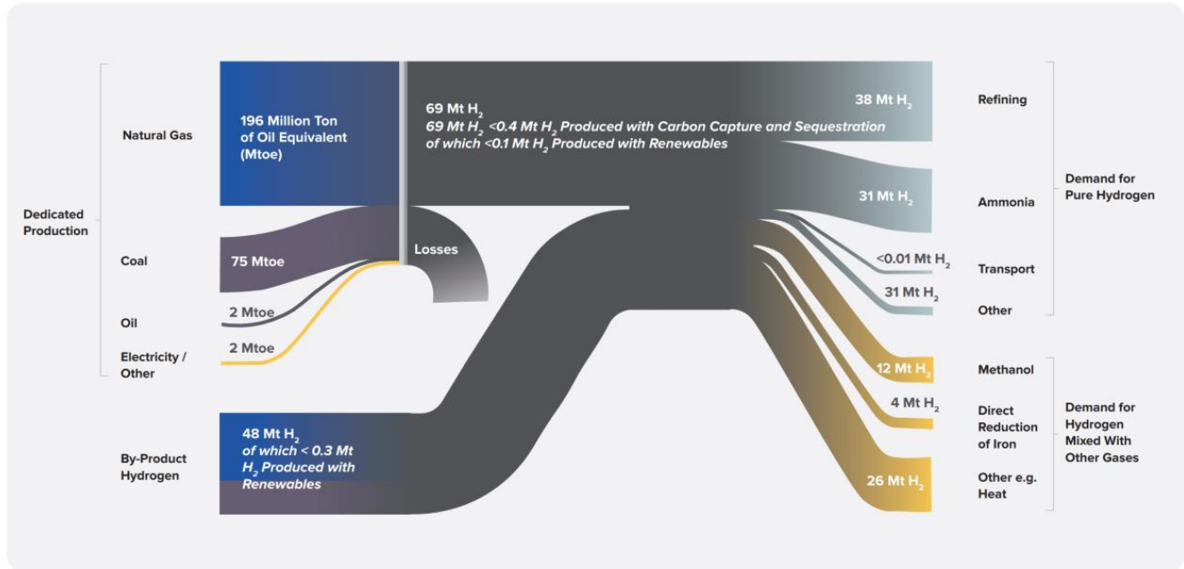
Figure 8: Global Hydrogen Production Sources and End Users 19
