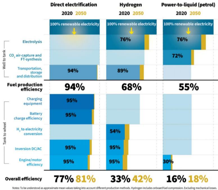
Figure 11: Electricity-to-Wheels Efficiency of Various Zero-Carbon Vehicle Pathways 61
