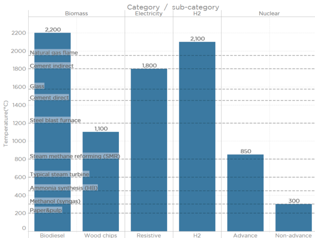
Figure 17: Temperature Requirements for Selected Industries and Temperature Available for Low-Carbon Heat Source Options 73
