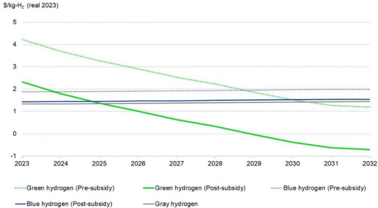
Figure 32: Forecasted Effect of Production Tax Credits on U.S. Levelized Cost of Hydrogen 131
