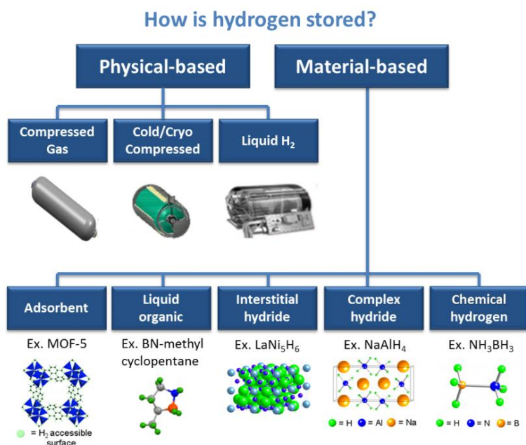
Figure 4: Hydrogen Storage Methods 35
