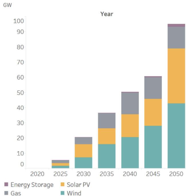
Figure 16: Forecasted Cumulative New Resource Build in the Northwest 66
