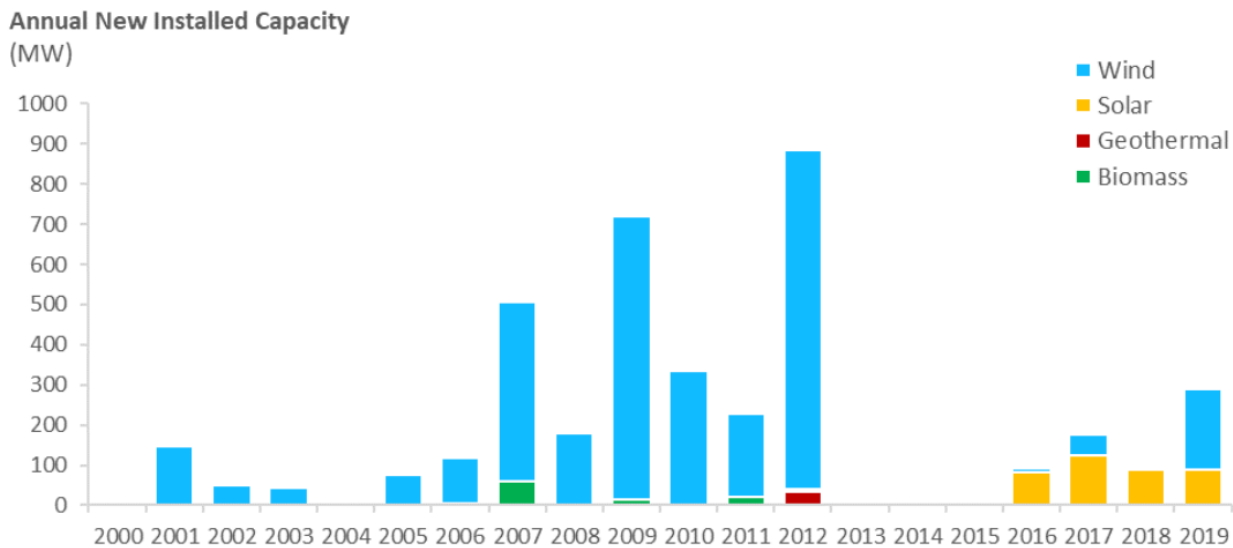
Figure 14: Annual Additions of Renewable Electricity Resources in Oregon Since 2000 65
