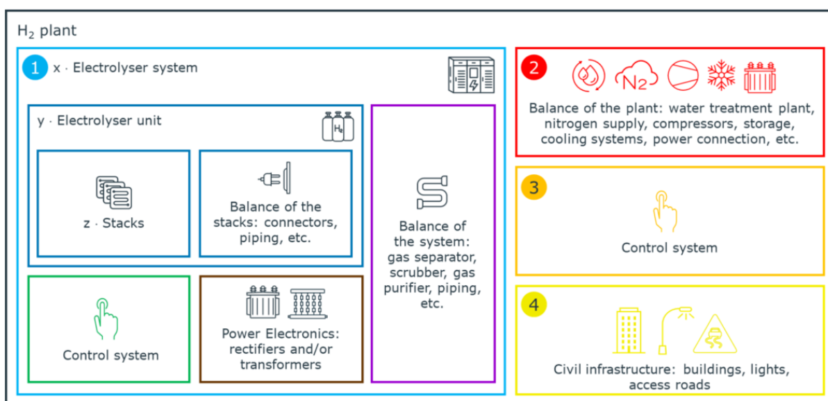
Figure 1 Hydrogen plant general components categorized into four main component groups: electrolyser system(s), balance of the plant, control system, and civil infrastructure.
