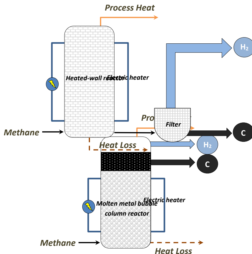
Figure 1. Thermal-assisted (heated-wall) Decomposition Diagram.
