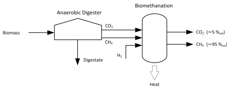
Figure 3: Simplified sketches of biogas plants illustrating the effect of biomethanation on energy and mass flows.
