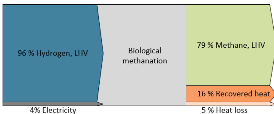
Figure 6: Energy balance of biological methanation (ex-situ).
