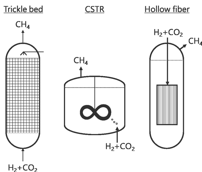
Figure 7. Examples of reactor design for biological methanation
