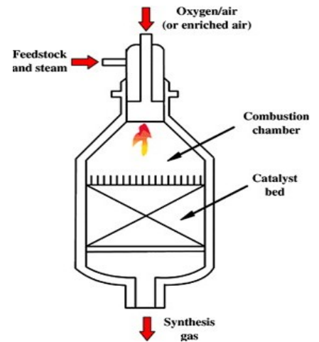
Figure 5: Autothermal reformer (ATR)
