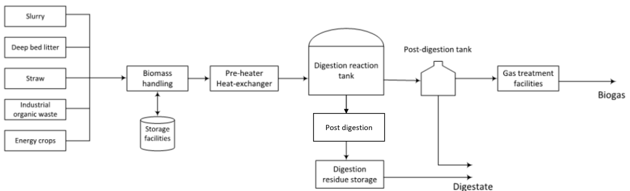
Figure 6: Typical components in a biogas plant. OBS alternative terms for technical description might be used by some actors: e.g., biomass handling might be referred to as pre-treatment, digestion reaction tank as a digester and digestion residue storage as digestate storage or post-storage of digestate.
