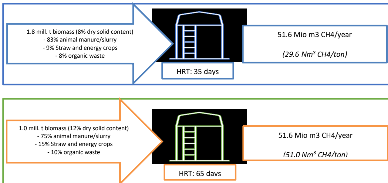
Figure 7: Biogas output in two different biogas plants – based on EUDPs very large plants (4a-A and 4b-A).
