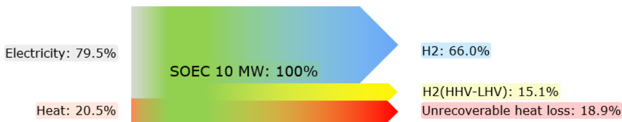
Figure 11 The energy inputs and outputs of an SOEC (2020, 10 MW hydrogen plants). Data is derived from Ramboll references.
