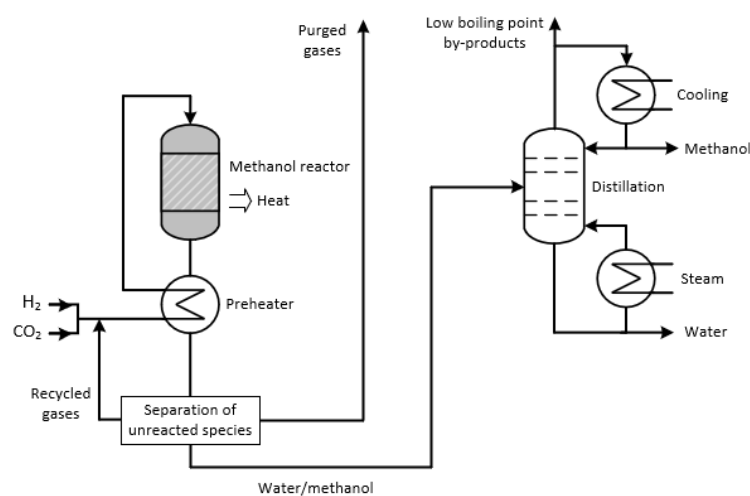
Figure 2: Simplified sketch of a hydrogen to methanol production plant.
