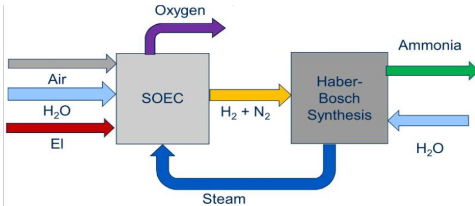
Figure 11: SOEC4NH 3 project combining electrolysis unit and ASU (EI = power)[ref 15]
