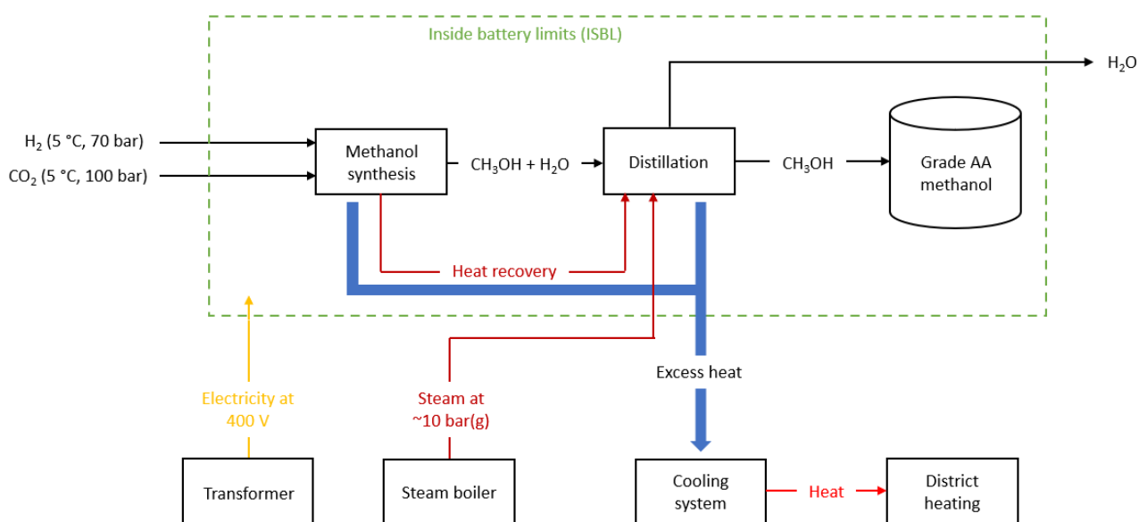
Figure 5: Illustration of battery limits.
