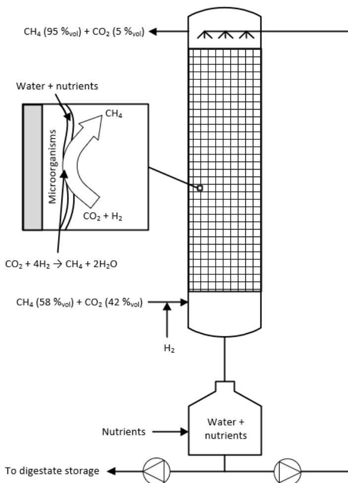
Figure 5: Sketch of a “trickle bed” biomethanation reactor. CSTR reactors have also been developed to near maturity (not shown).
