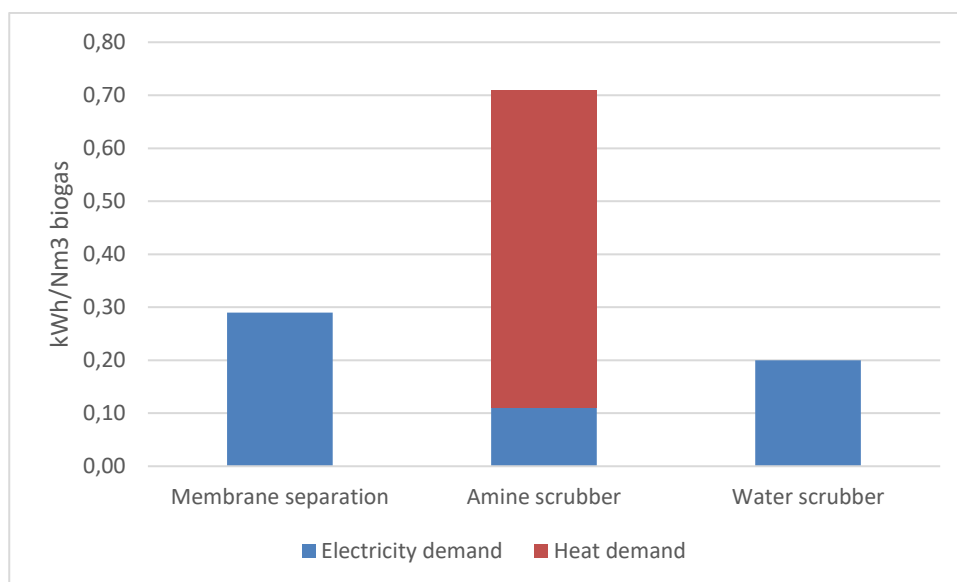
Figure 12: Energy consumption (kWh/Nm 3 raw biogas) for the upgrading technologies, water scrubbing, amine scrubber and membrane
