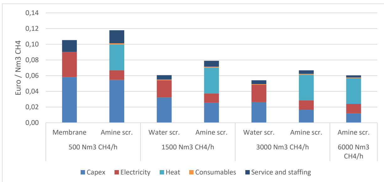
Figure 11: Comparison of the cost of upgrading biogas (excluding the cost of the biogas plant) using different upgrading technologies at plants of different scales. The calculation assumes 50% reuse of the waste heat (assuming 80% reuse the amine scrubbers are the cheapest per Nm 3 ). The results are based on a private sector stakeholder perspective assuming a 10% discount rate. In the calculations, the price for electricity is 6.3 Euro/100 kWh Source: Calculations by Ea Energy Analyses based on [9]
