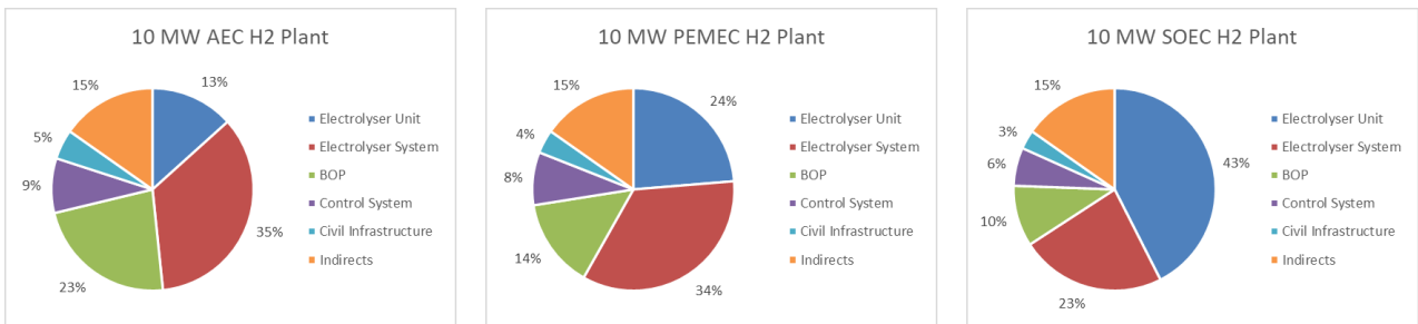
Figure 17 Cost breakdown of a 10 MW hydrogen plant for (left) AEC, (middle) PEMEC, and (right) SOEC.
