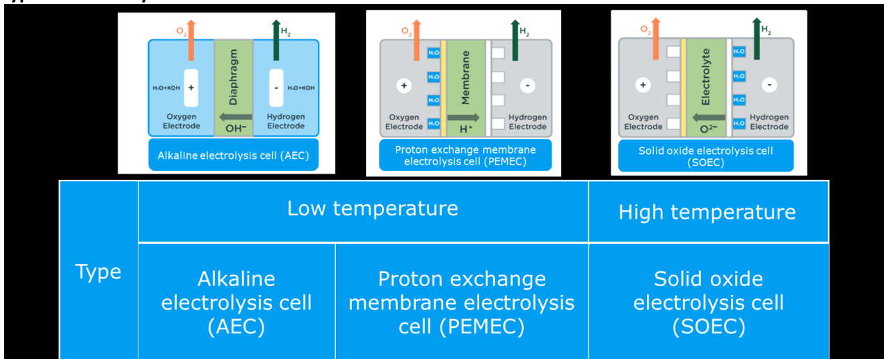
Figure 4 The three primary electrolyser technologies: AEC, PEMEC, and SOEC.
