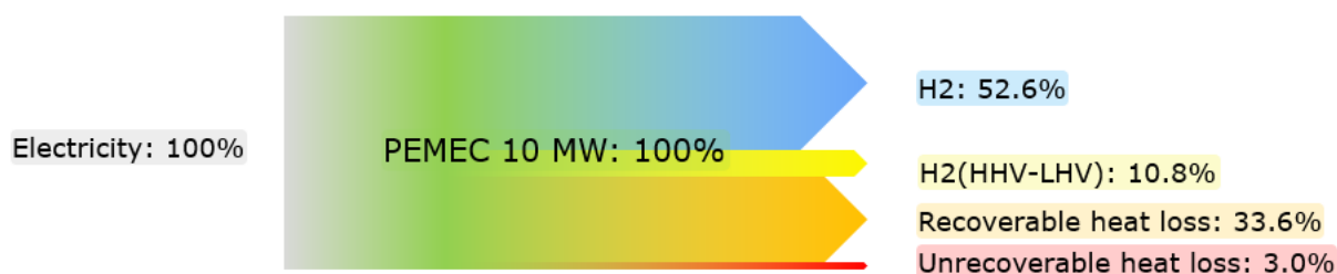
Figure 10 The energy inputs and outputs of a PEMEC (2020, 10 MW hydrogen plants). Data is derived from Ramboll references.
