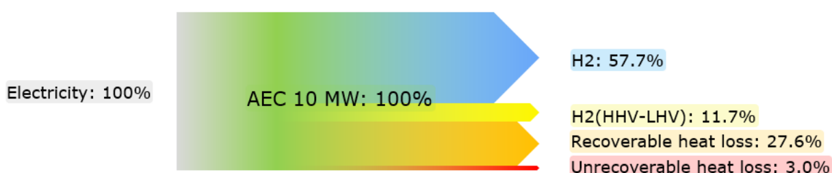
Figure 9 The energy inputs and outputs of an AEC (2020, 10 MW hydrogen plants). Data is derived from Ramboll references.
