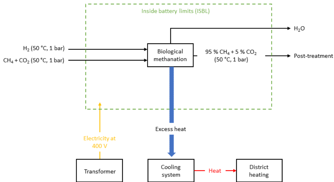
Figure 8: A sketch indicating the assumption on battery limits used for generating the performance and cost for the data sheet.
