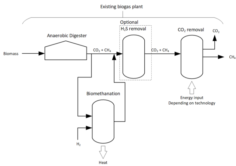
Figure 4: Integration examples of biomethanation (ex-situ) in existing biogas plants. Data from some suppliers indicate that grid level biomethane could be achieved directly after the biomethanation reactor, meaning the CO 2 removal unit and H 2 S unit could be optional and omissible to save costs. This has been proven in demonstration scale. Water vapor is also removed prior to injection the methane on the grid (not shown).
