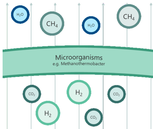
Figure 2: Microorganisms in a biomethanation process where hydrogen and carbon dioxide react to form methane and water.
