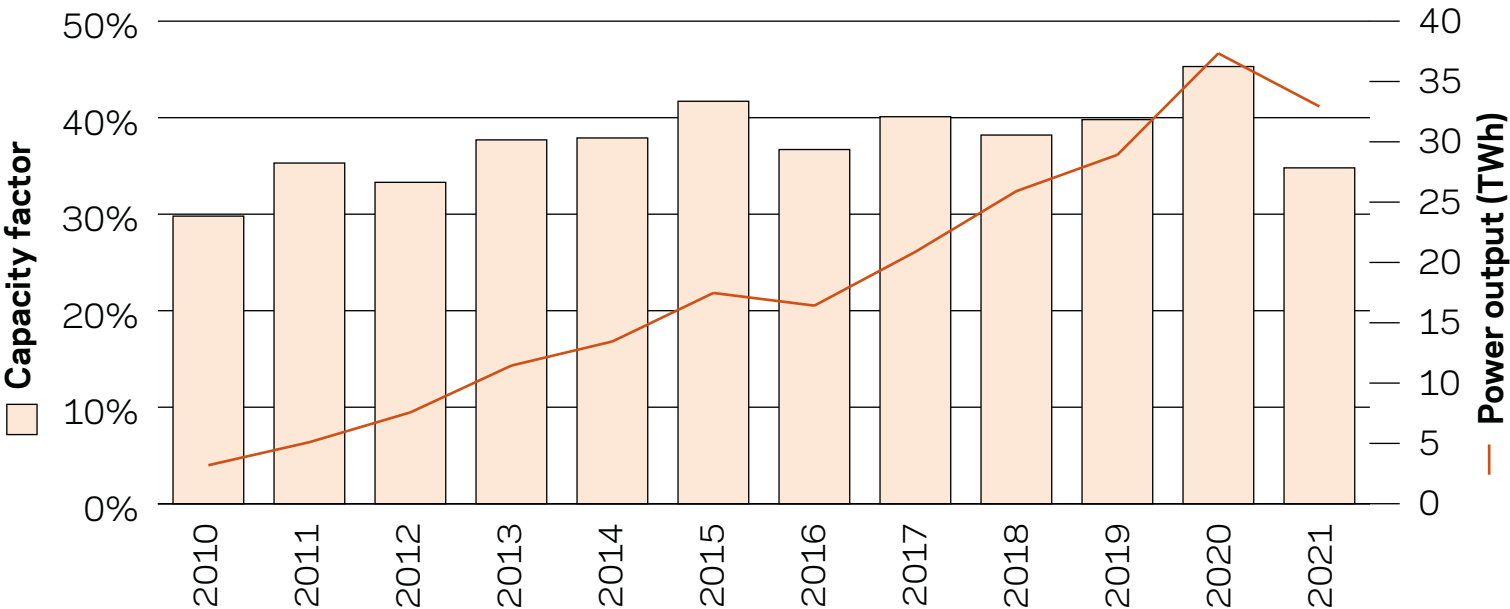
Figure 9: Capacity factor - England & Wales
