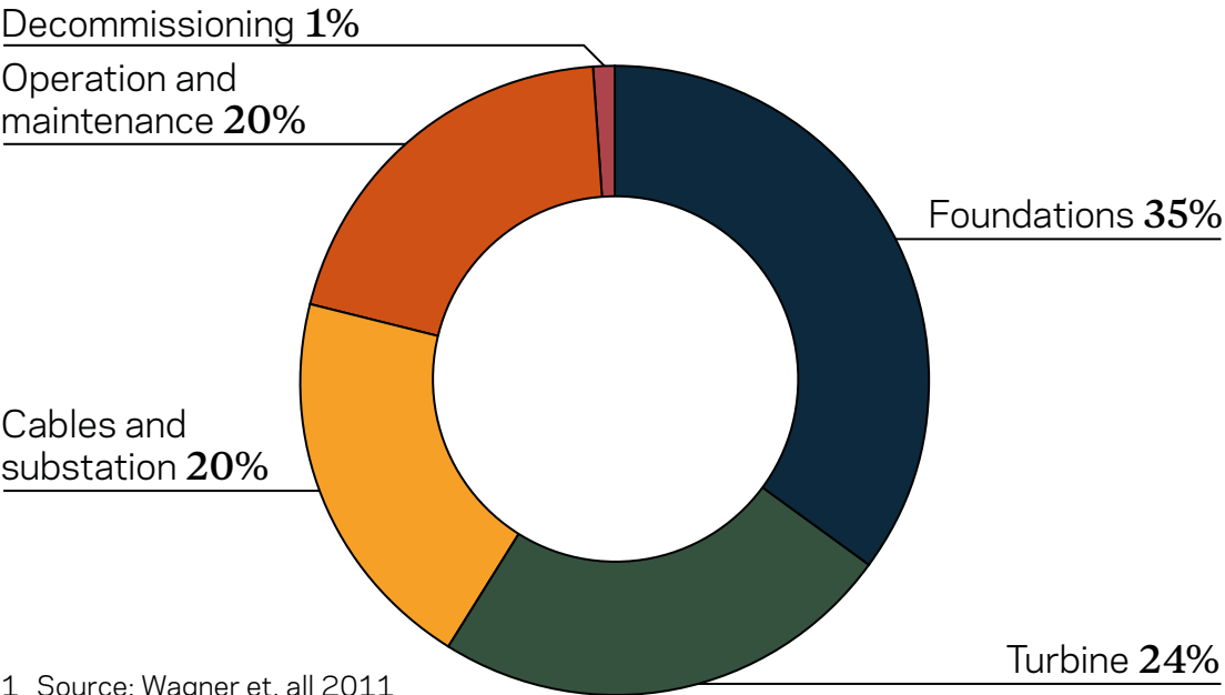
Figure 17: Breakdown of carbon emissions for an offshore wind farm 1
