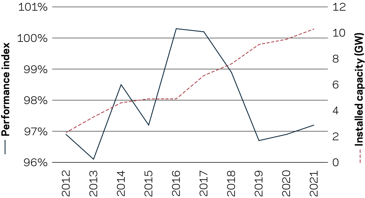
Figure 10: Fleet Performance Index - England and Wales
