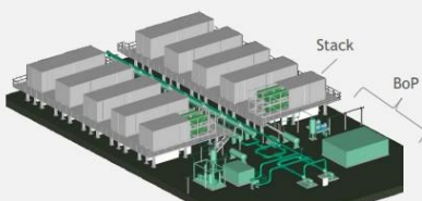
Battolyser 3 impression (~10MW)
