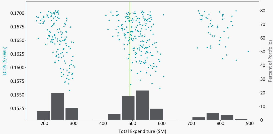
Figure 5. LCOS and expenditures for the top 10% of the portfolios for hydrogen with surface tank storage. The axis on the left labels the scatterplot of expected LCOS for each portfolio versus total expenditure, while the axis on the right labels the histogram of expenditures. This means that the histogram shows the distribution of the dots on the scatterplot. The vertical line marks the median expenditure.
