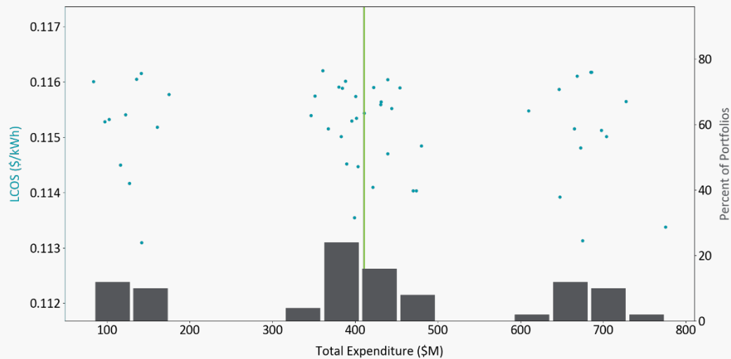
Figure 6. LCOS and expenditures for the top 20% of the portfolios for hydrogen with salt cavern storage. The axis on the left labels the scatterplot of expected LCOS for each portfolio versus total expenditure, while the axis on the right labels the histogram of expenditures. This means that the histogram shows the distribution of the dots on the scatterplot. The vertical line marks the median expenditure.
